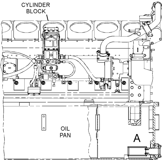
RIGHT SIDE VIEW OF ENGINE
