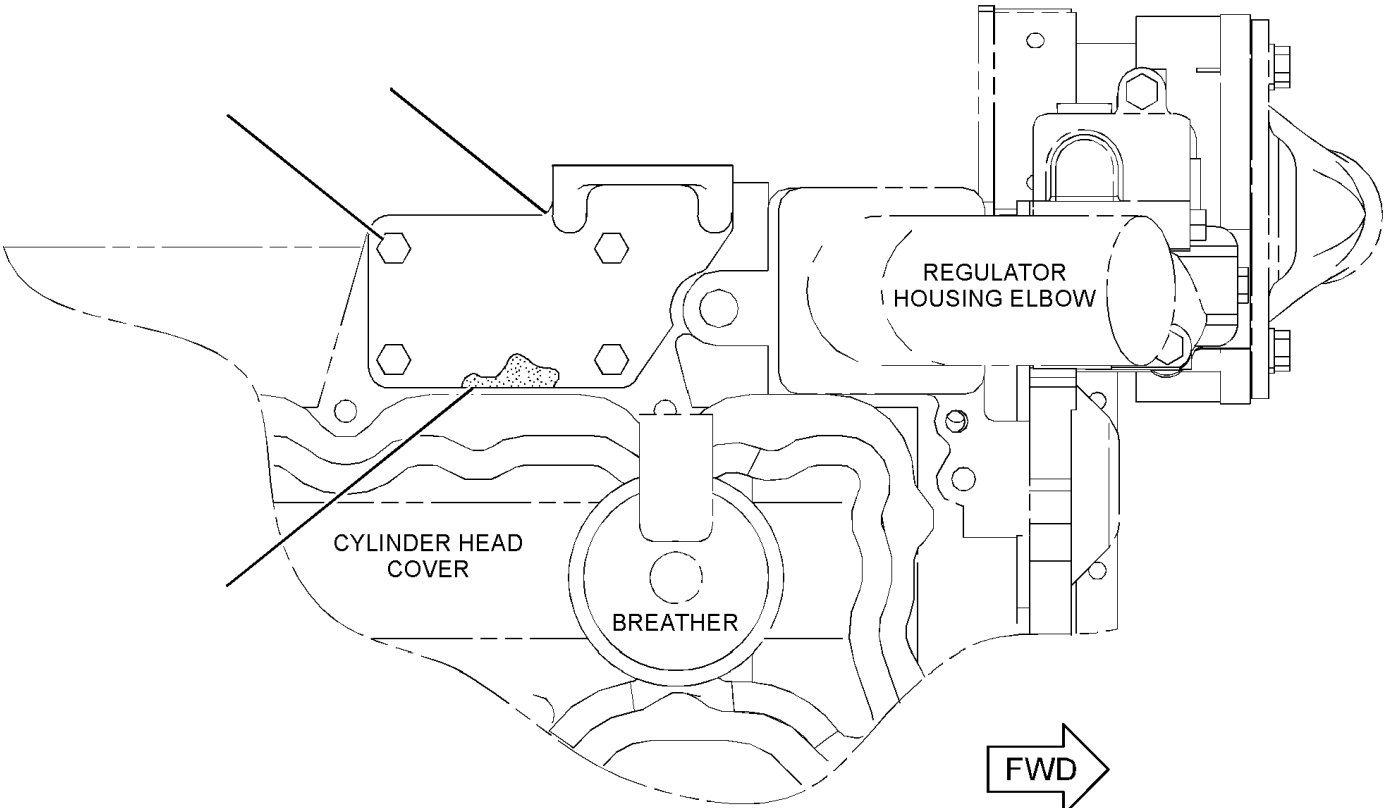
TOP VIEW
