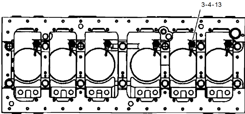
BOTTOM VIEW OF ENGINE
