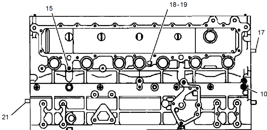
RIGHT SIDE VIEW OF ENGINE
