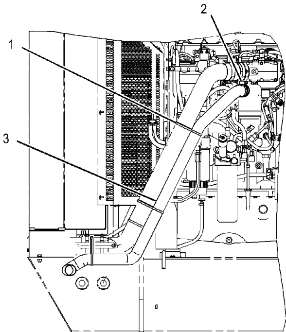
LEFT SIDE VIEW OF ENGINE (NARROW BASE)
