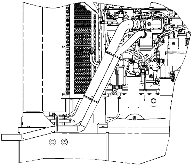
LEFT SIDE VIEW OF ENGINE (WIDE BASE)
