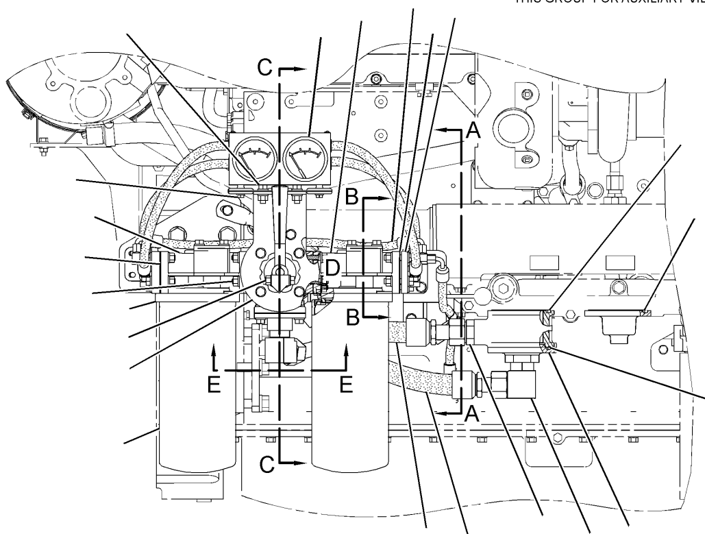
RIGHT SIDE VIEW OF ENGINE
