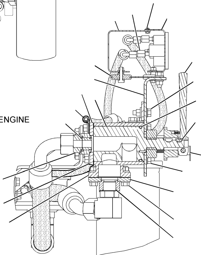
SECTION C-C
