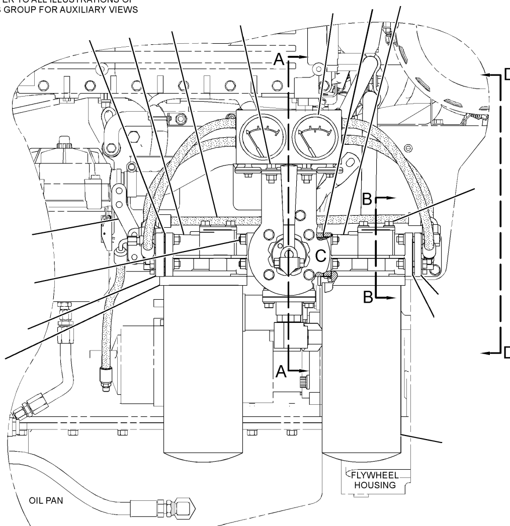
LEFT SIDE VIEW OF ENGINE
