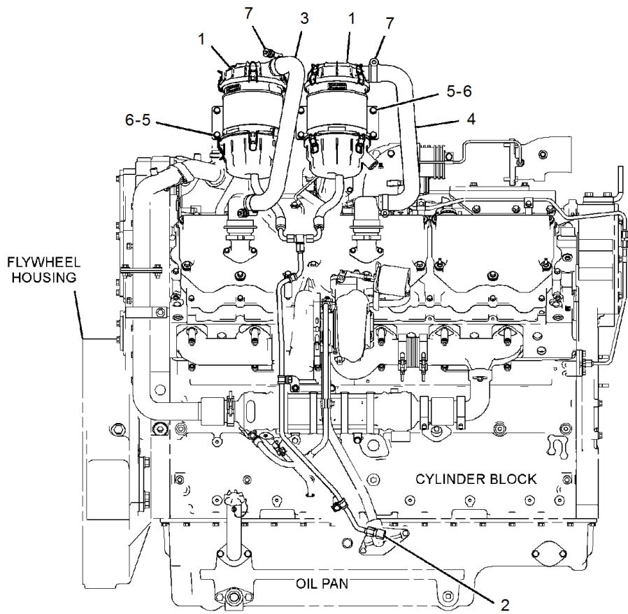
RIGHT SIDE VIEW OF ENGINE
