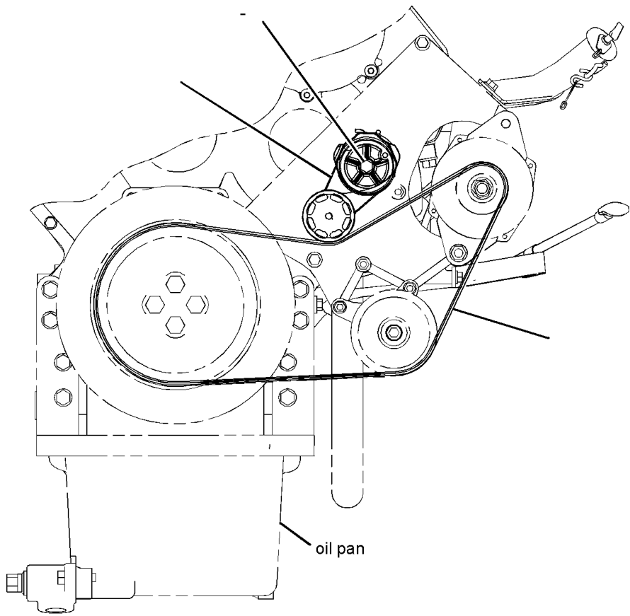
FRONT VIEW
