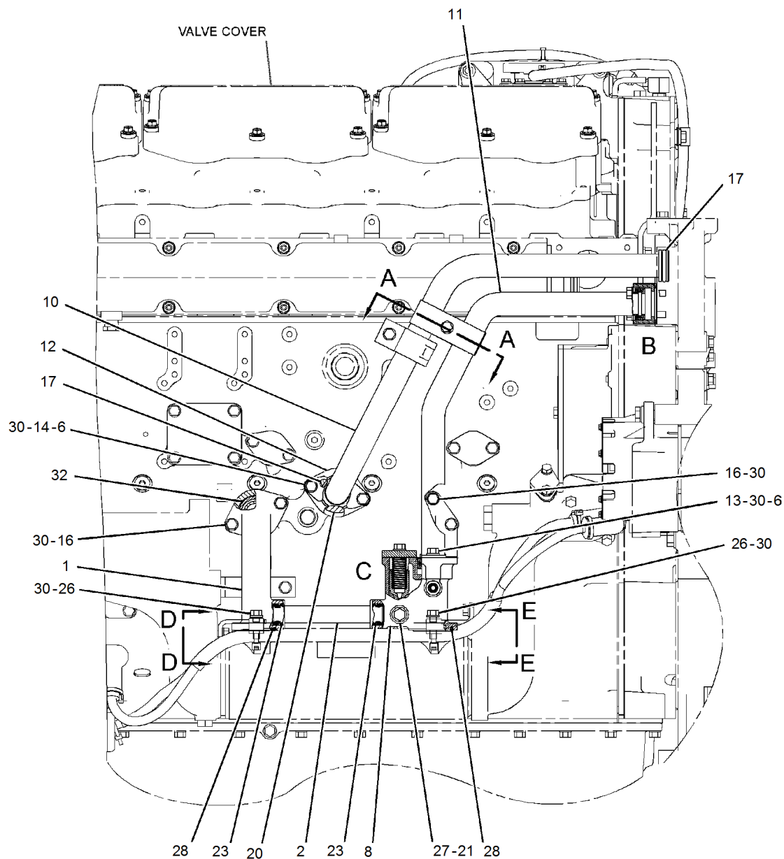
RIGHT SIDE VIEW OF ENGINE
