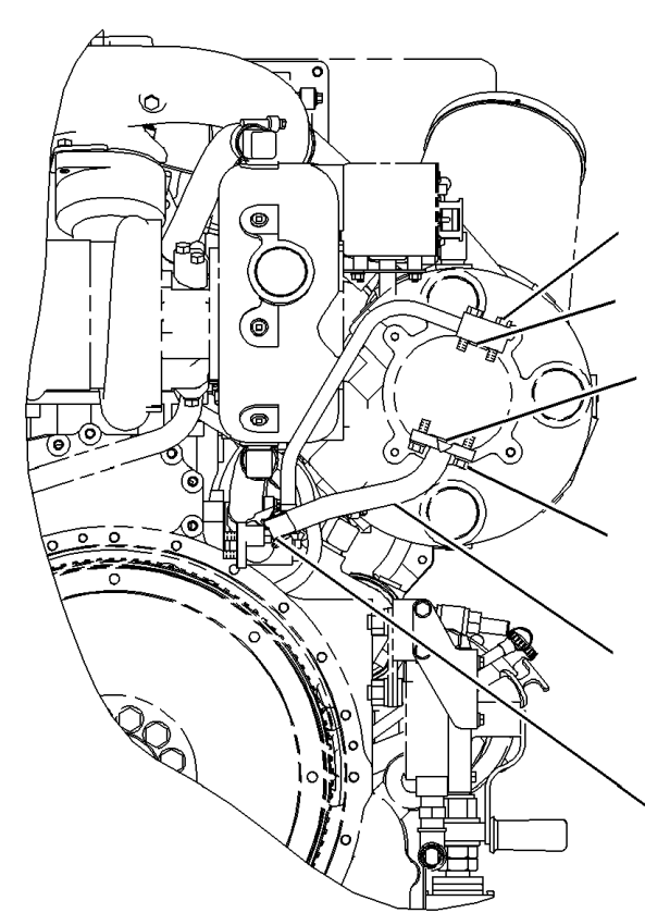
REAR VIEW
