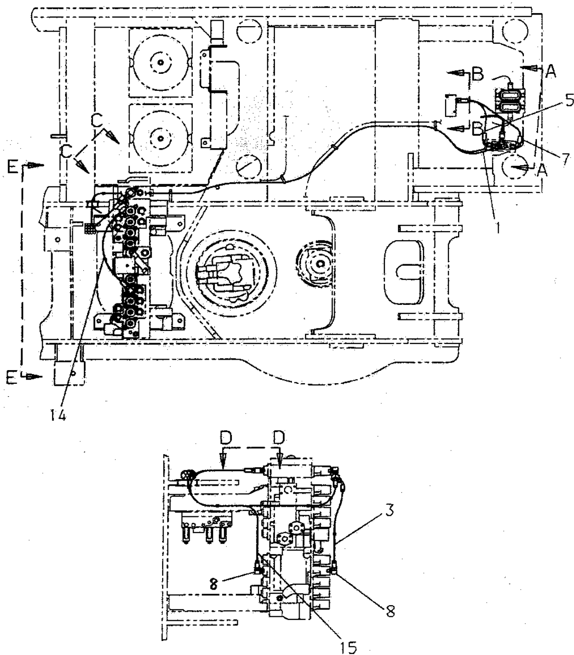
VIEW E-E
