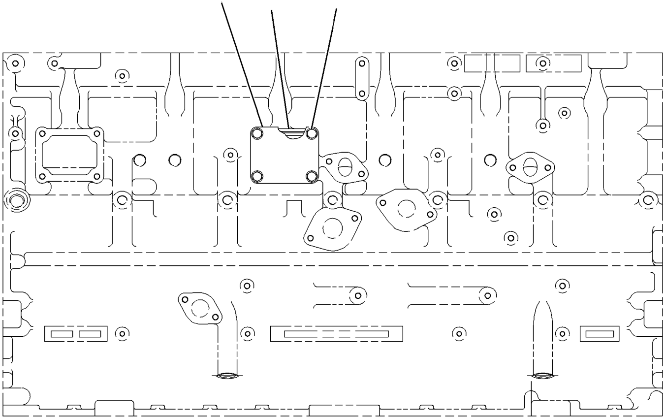
Drawing 1 of 1
