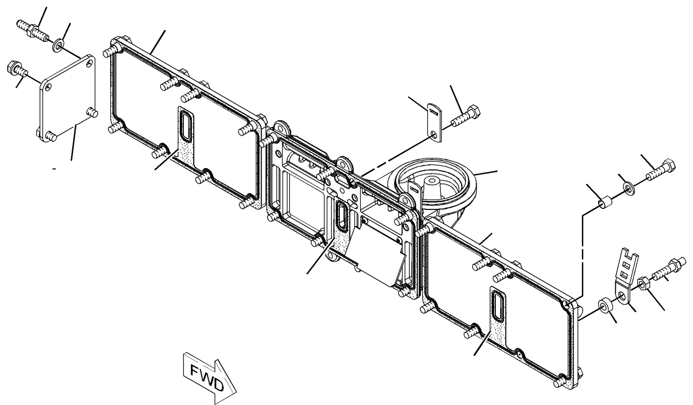
Drawing 1 of 1
