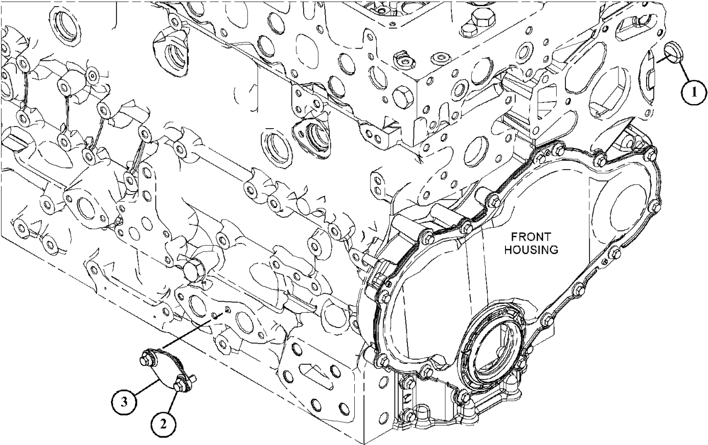
Drawing 1 of 1
