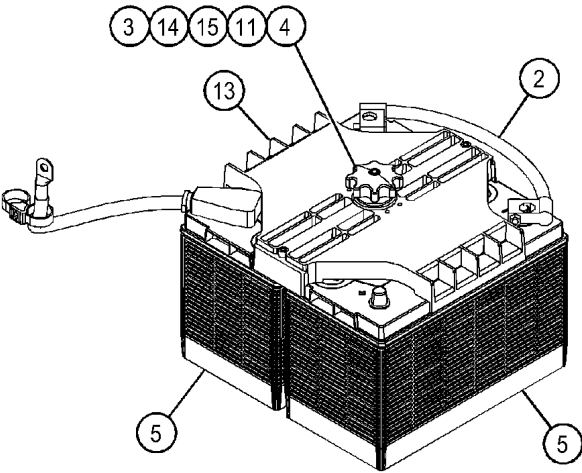
VIEW OF AREA A (PARTS REMOVED FOR CLARITY)
