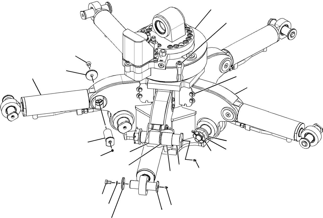
Drawing 1 of 1
