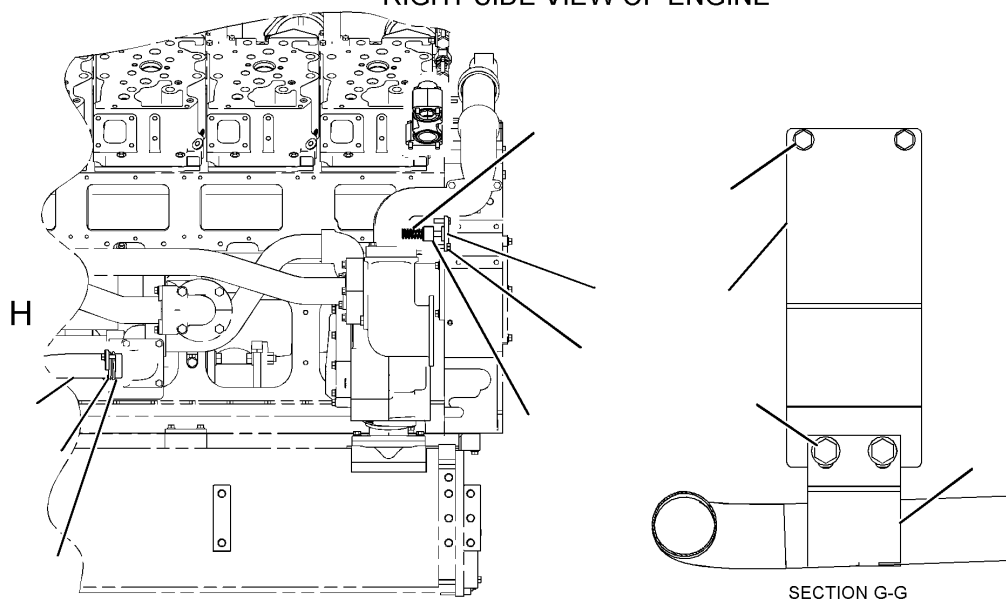
SECTION G-G
