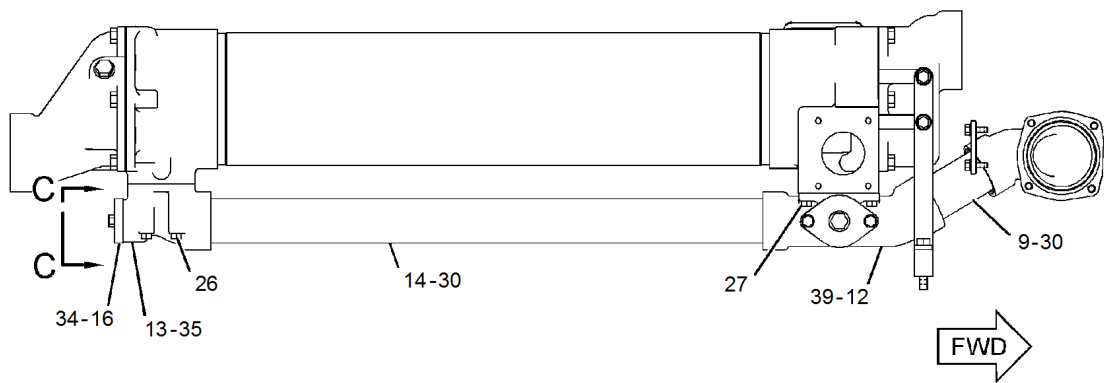
BOTTOM VIEW
