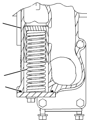
SECTION C-C
