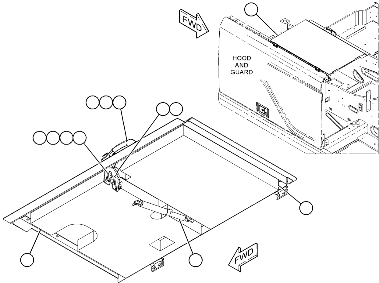
Drawing 1 of 1
