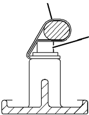
SECTION C-C
