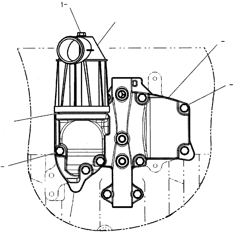
LEFT SIDE OF ENGINE
