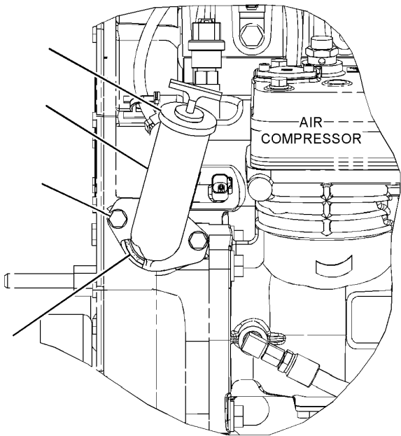
LEFT SIDE VIEW OF ENGINE
