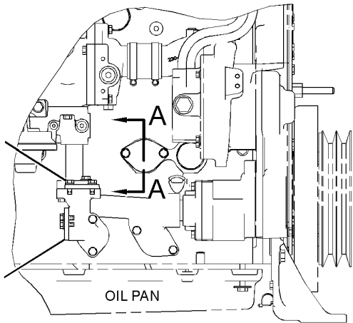
RIGHT SIDE VIEW OF ENGINE
