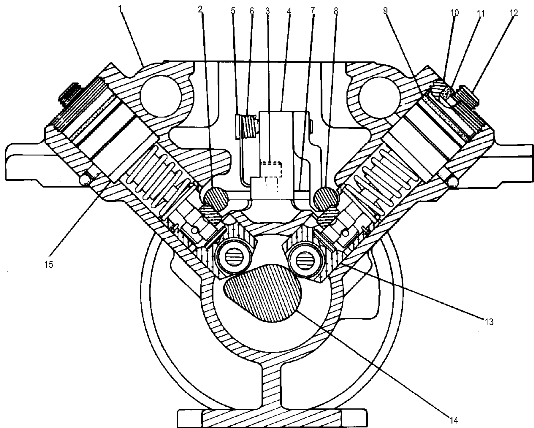
SECTION B-B
