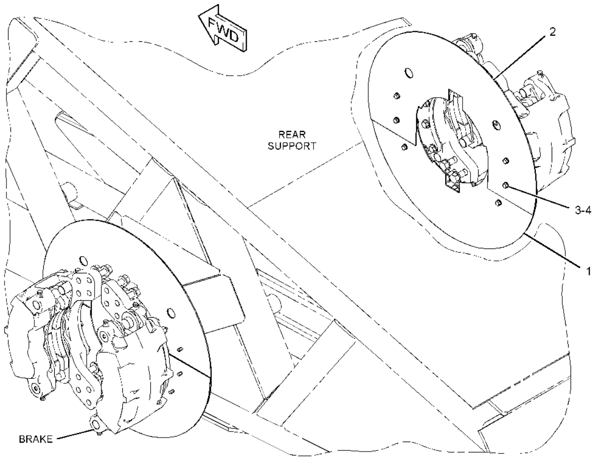
Drawing 1 of 1
