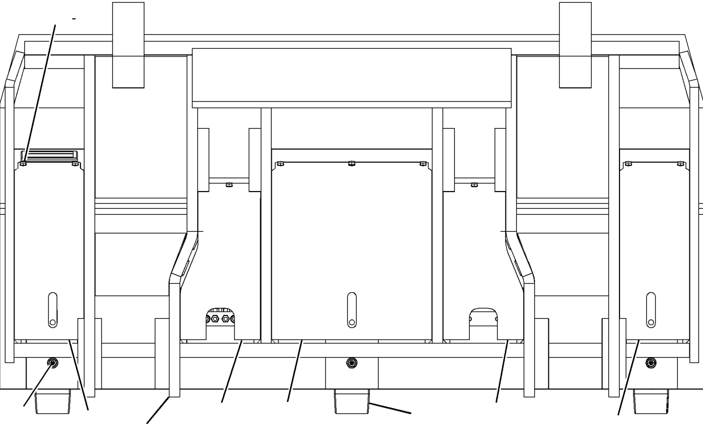
REAR VIEW
