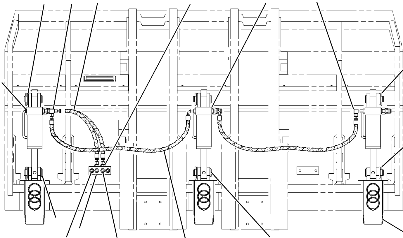
REAR VIEW
