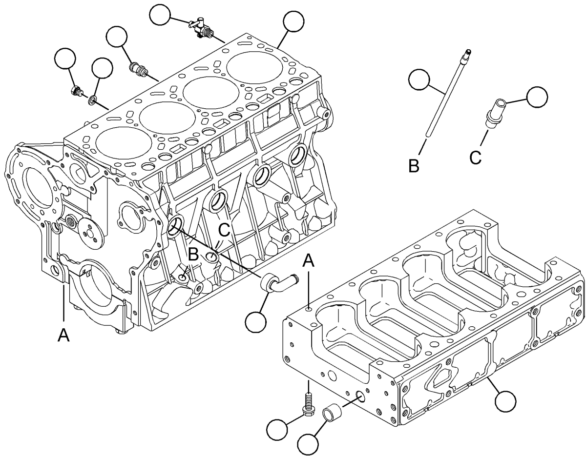
Drawing 1 of 1
