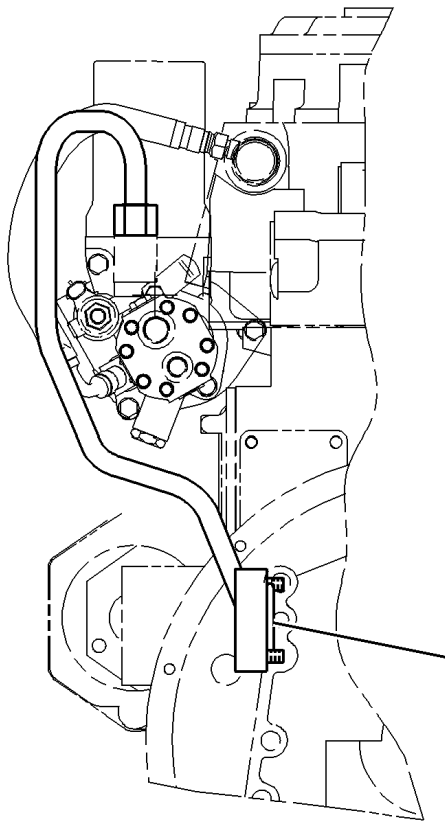
REAR VIEW
