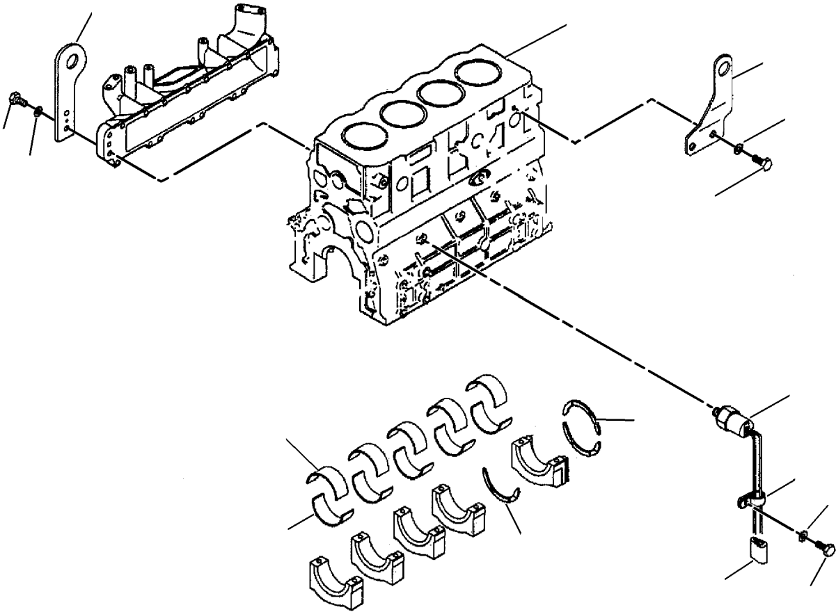
Drawing 1 of 1
