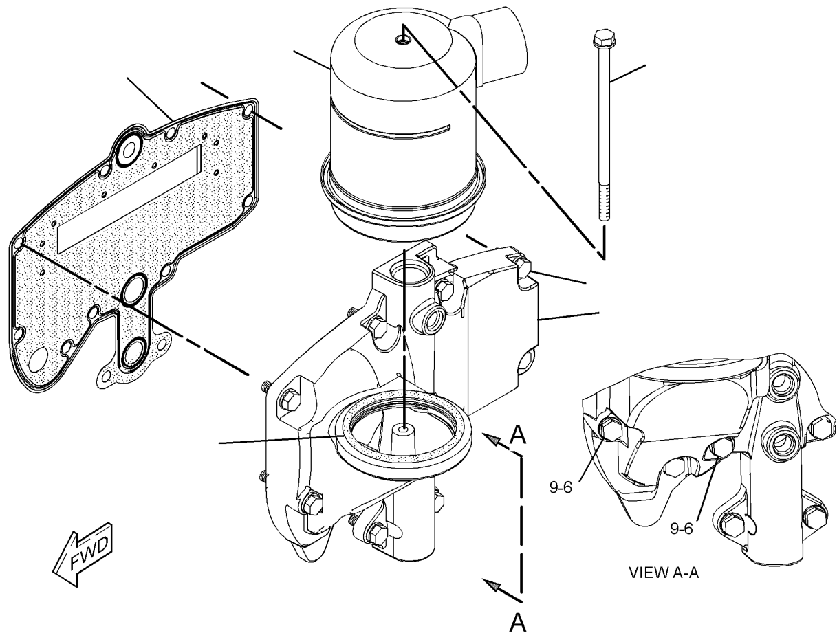
Drawing 1 of 1
