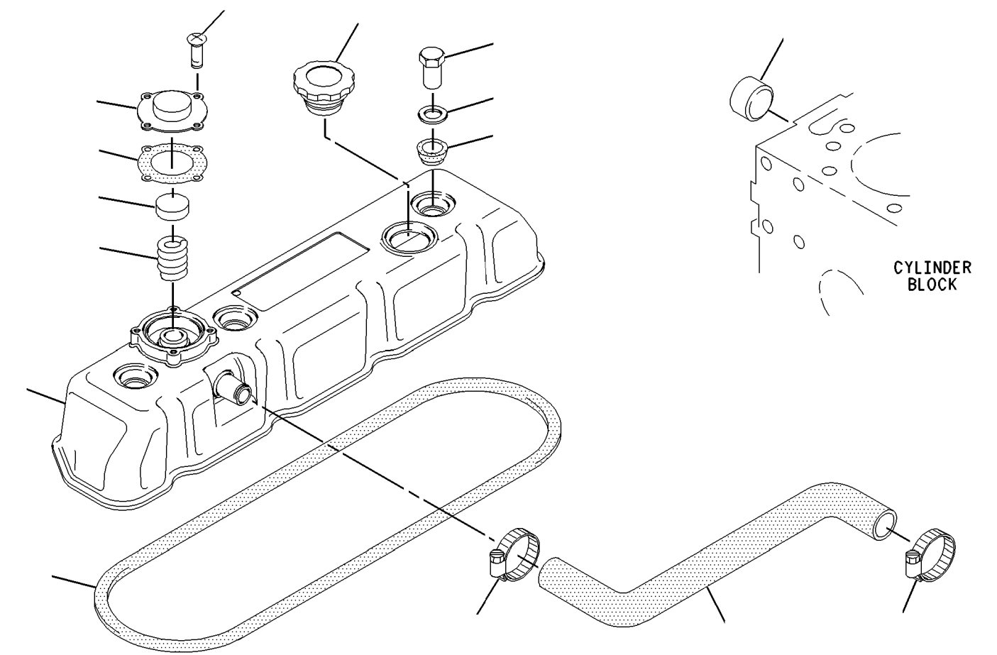
Drawing 1 of 1
