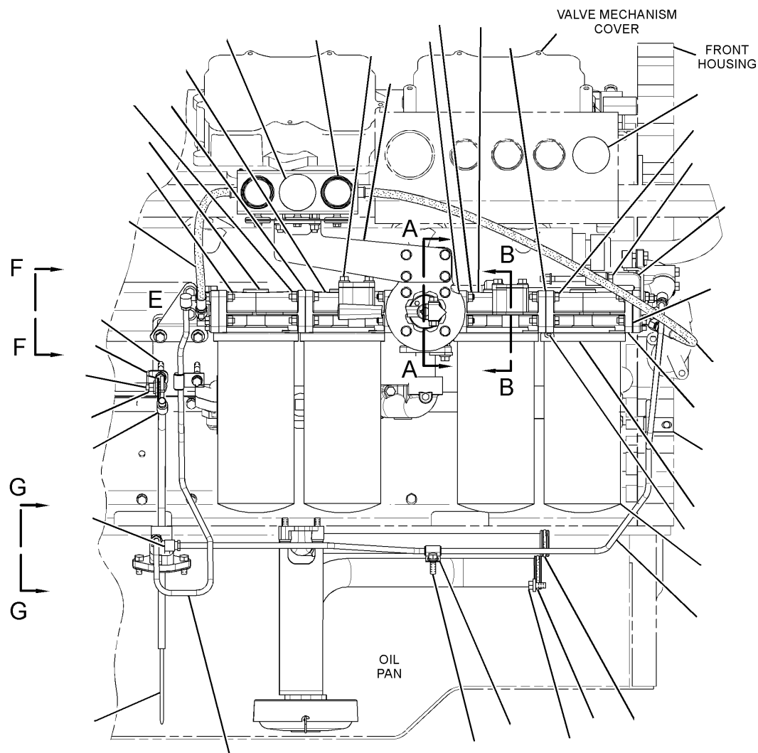
RIGHT SIDE VIEW OF ENGINE
