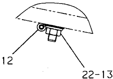
SECTION G-G
