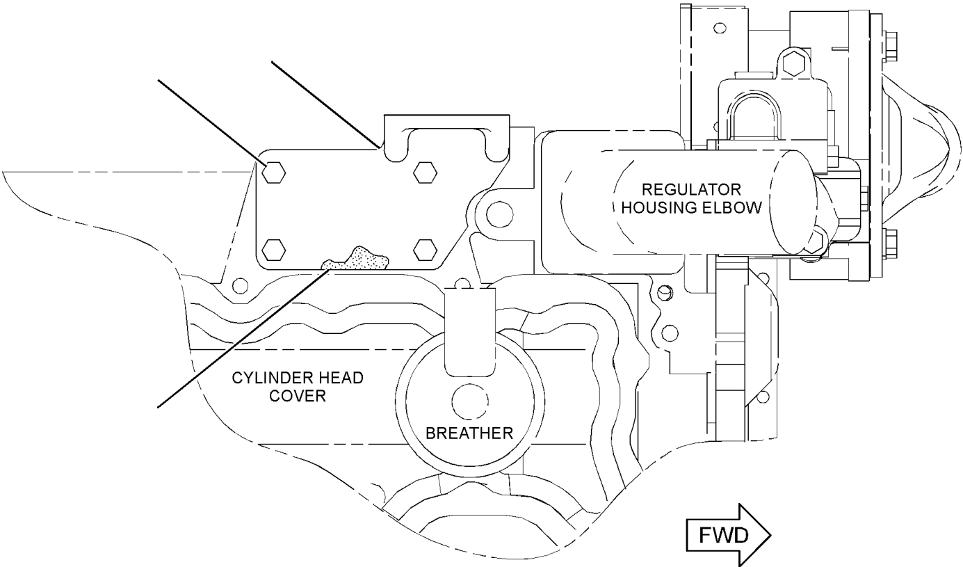
TOP VIEW
