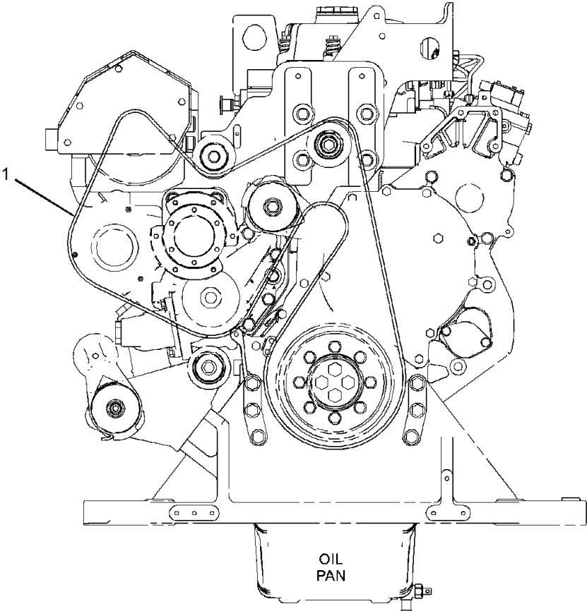
FRONT VIEW OF ENGINE
