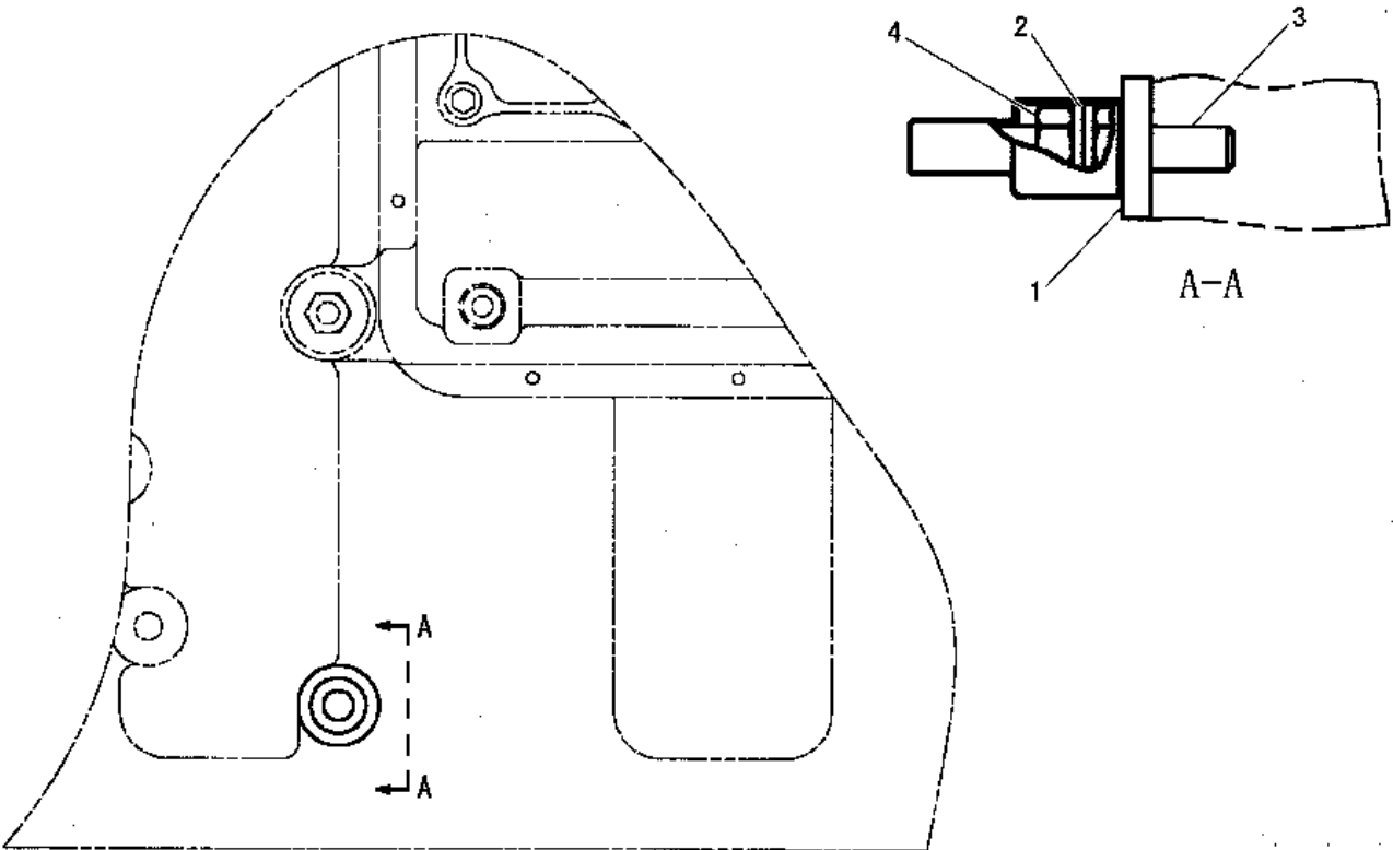
LEFT SIDE OF ENGINE
