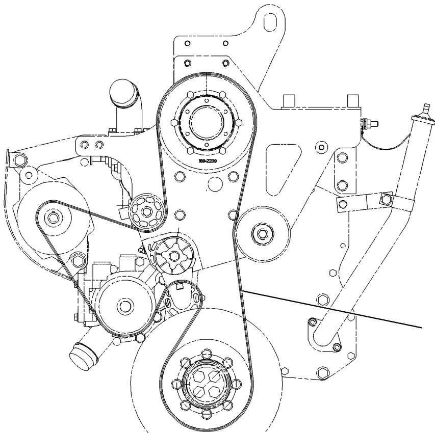
FRONT VIEW OF ENGINE
