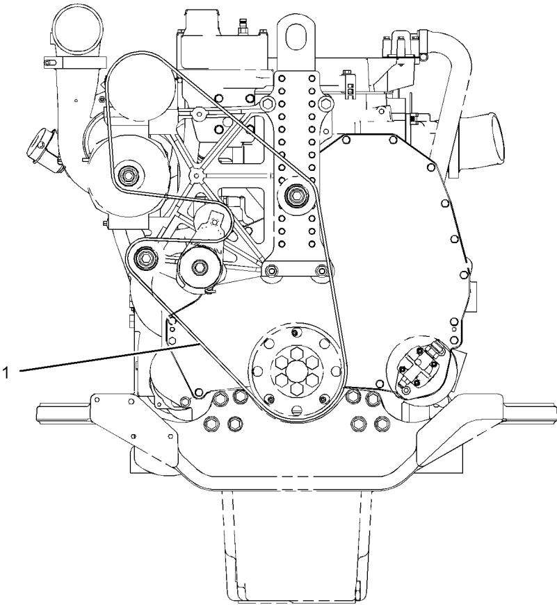
FRONT VIEW
