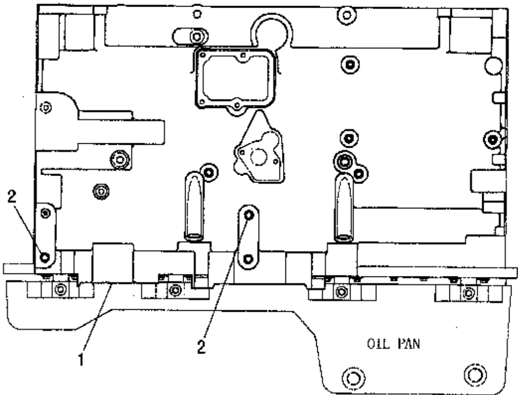
LEFT SIDE OF ENGINE
