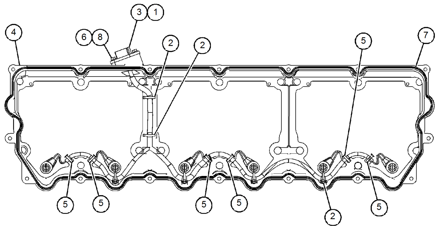
BOTTOM VIEW OF ENGINE
