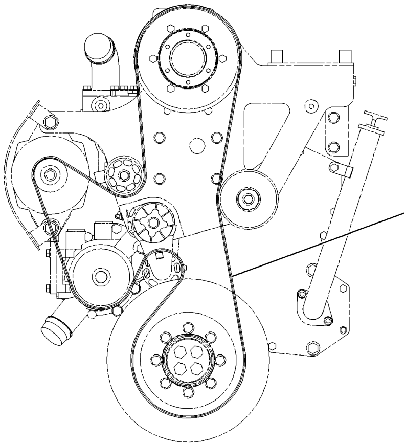
FRONT VIEW OF ENGINE
