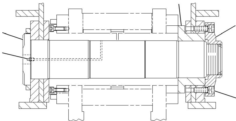
SECTION C-C
