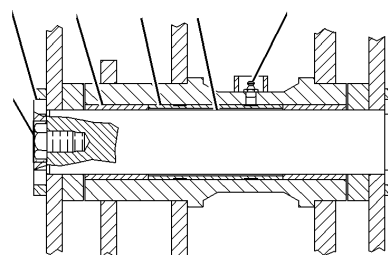
SECTION F-F
