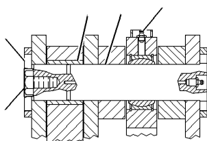
SECTION E-E
