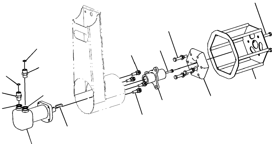
VIEW OF AREA A (EXPLODED)
