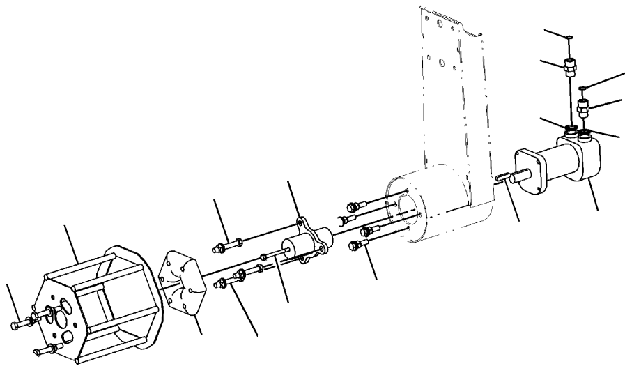
VIEW OF AREA B (EXPLODED)
