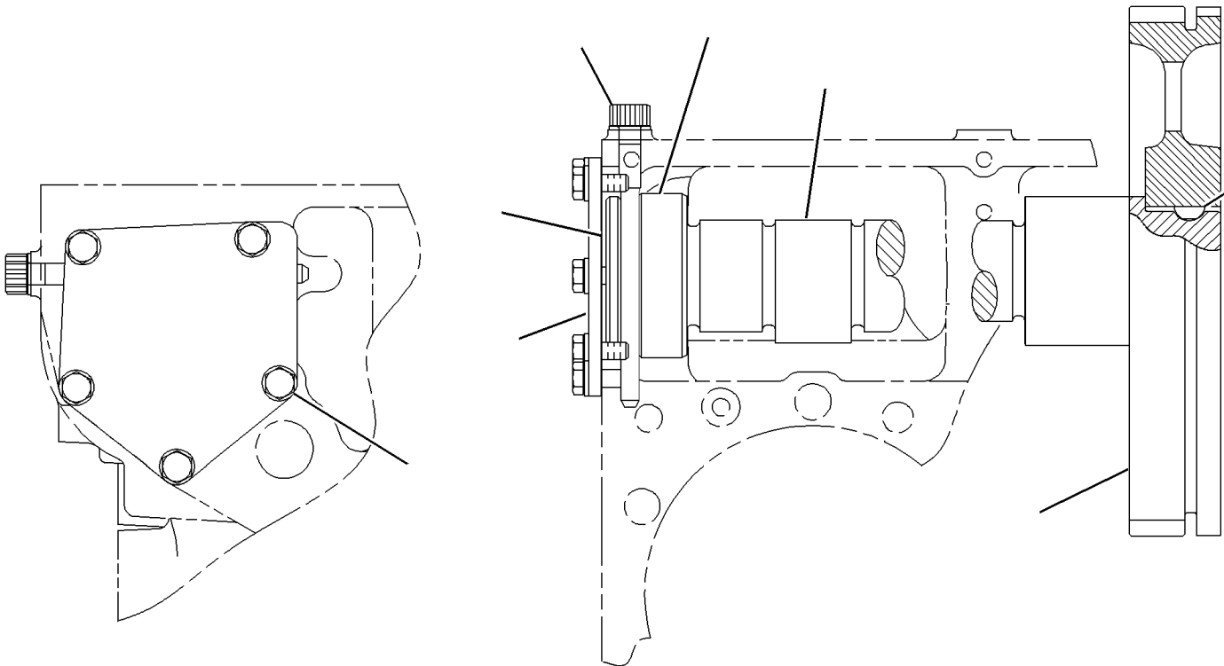
REAR VIEW
