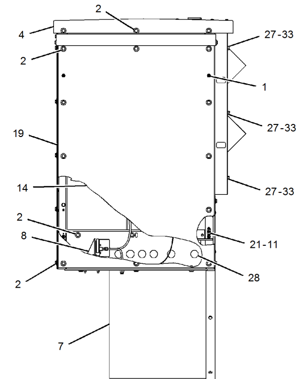
VIEW C-C
