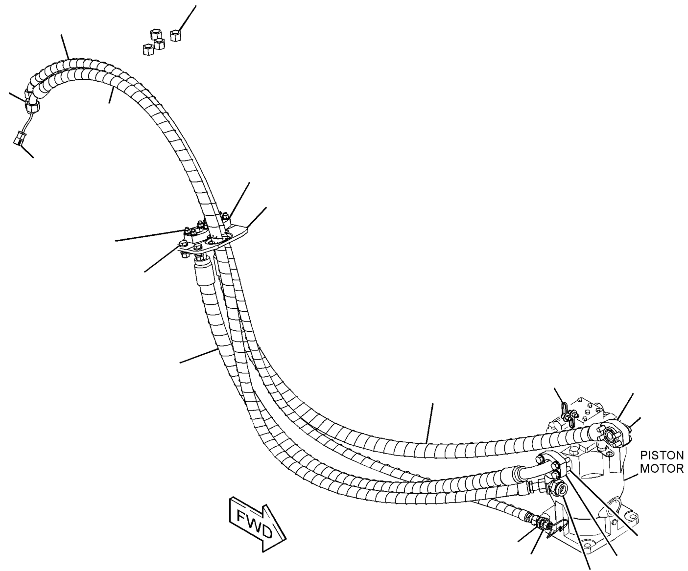
Drawing 1 of 1
