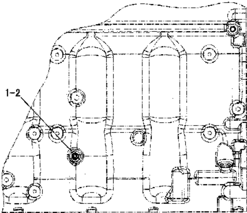
LEFT SIDE OF CYLINDER BLOCK
