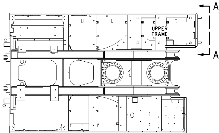
TOP VIEW
