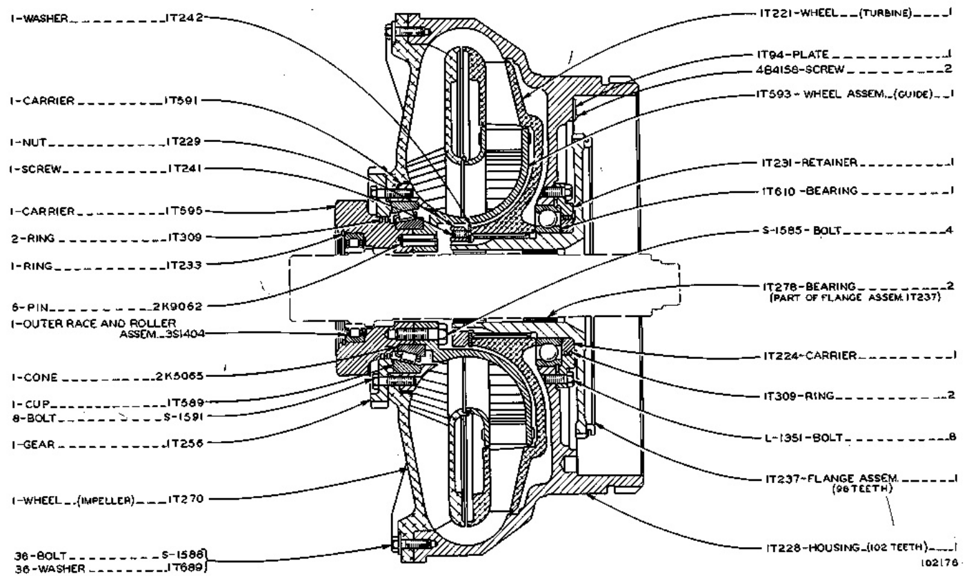
Drawing 1 of 1
